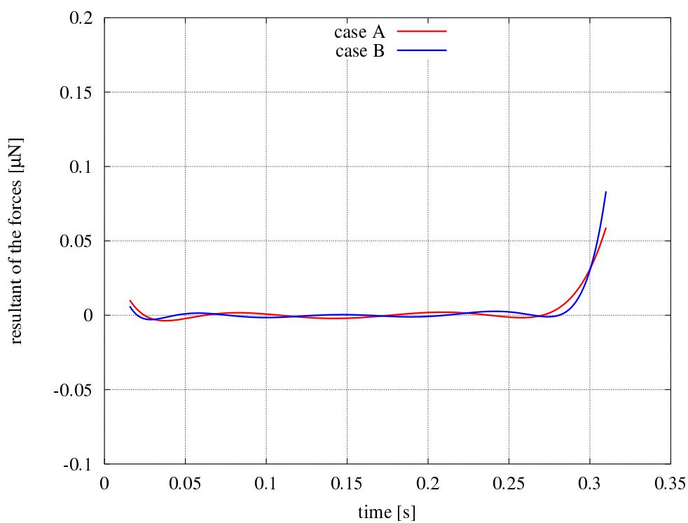
Figure E.6: Resultant of the liquid inertia forces for two different set of polynomial data fit for the volume and the center of gravity of the bubble.
