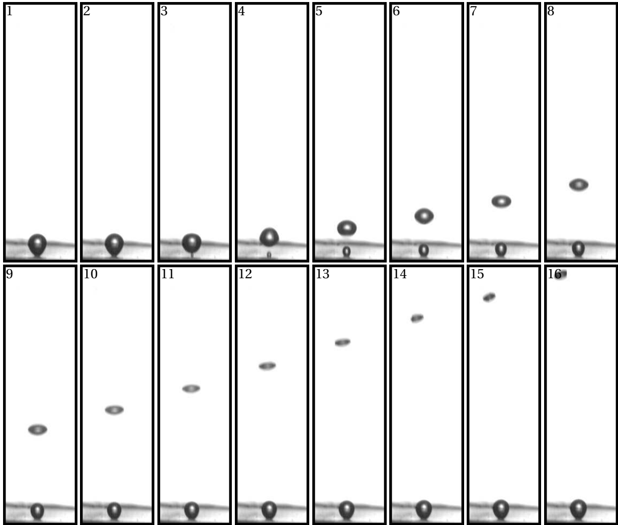
Figure 5.70: Photos of a typical bubble rise, at a wall superheat of \Delta T_W \approx 3.5 K. Time difference between two photos is \Delta t = 2.5 ms. Physical height represented is \Delta z \approx 14 mm.
