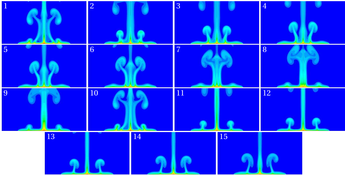
Figure 4.12: Temperature field at q = 5 \text{ kW} \cdot \text{m}^{-2} using C3. \Delta t = 800 \text{ ms} between successive images.
