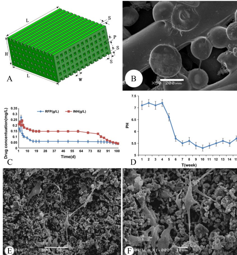
Fig. 12. \beta -TCP scaffolds loaded with Rifampin and Isoniazid. (A) Scaffold model (S=P=500 \mu\text{m} ; W=400 \mu\text{m} ; H=5 mm; L=11.3 mm). (B) SEM image of drug-loaded \beta -TCP support with microspheres (50x). (C) In vitro drug release profile. (D) pH change of SBF over time as the scaffold degrades. (E) 500x and (F) 1000x SEM images of rBMSC adhesion to the scaffold.
