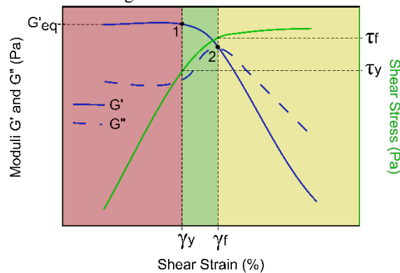
Fig. 24. Schematic illustration of the evolution of storage ( G' ) and loss ( G'' ) moduli and shear stress with increasing shear strain showing the three different areas and the values of interest.
