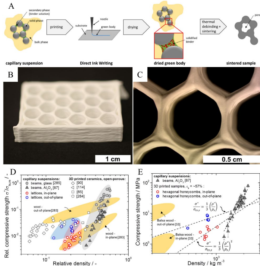
Fig. 10. \alpha -Alumina scaffolds from capillary suspensions inspired in balsa wood [88]. (A) Schematic illustration of the processing route with the open-porous structure of the sintered struts being based on the open-porous network of capillary suspension that serves as a precursor for the ceramic part. (B) and (C) Hexagonal honeycomb structures. (D) Relative compressive strength vs. relative density for honeycomb scaffolds and other 3D printed ceramics and glasses with fully open-porous struts. \sigma_{ts,m} : tensile strength of the matrix. (E) Compressive strength as a function of density. The graph shows data for honeycomb scaffolds with constant strut porosity ( \epsilon_s ) of \sim 57\% and slip-cast specimens based on capillary suspensions [87]. The dependence of strength on the density of the 3D printed samples fits well with the scaling laws for in-plane and out-of-plane loaded hexagonal honeycomb structures [89].
