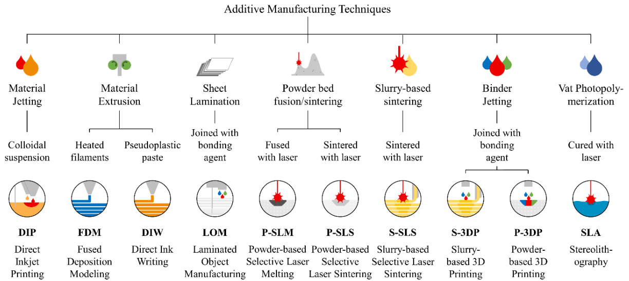
Fig. 2. Schematic representation of the additive manufacturing techniques most used for ceramics.
