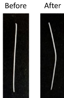
Fig. 54. Photograph of a CS-ATZ filament that had been printed with a 410 \mu\text{m} nozzle before and after undergoing cycles of deformation. It is possible to observe the expressive inelastic deformation presented by the CS-ATZ filaments after 3PB and before fracture.
