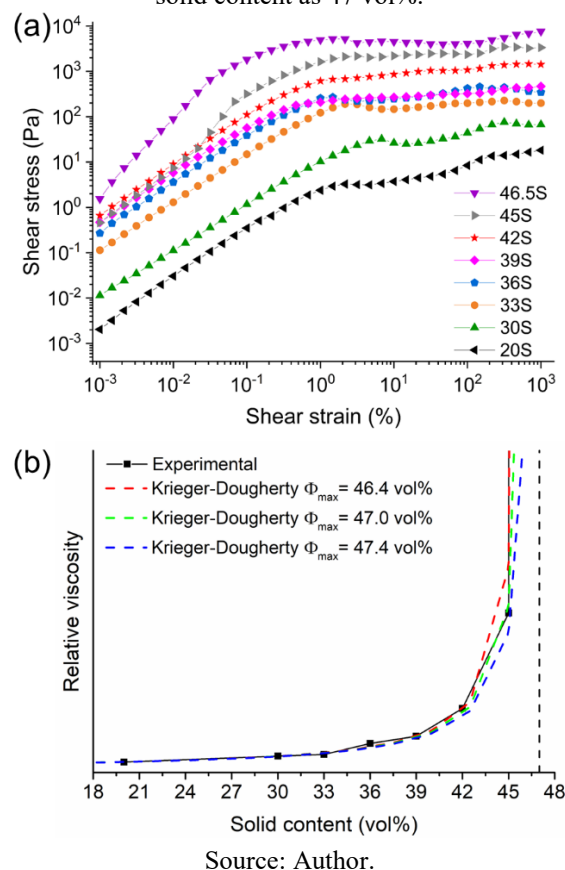
Fig. 29. Determination of the maximum solid content. (a) Shear stress vs. shear strain for pastes with different solid contents. (b) Fitting of Krieger-Dougherty curves with the experimental values, establishing the maximum solid content as 47 vol%.
