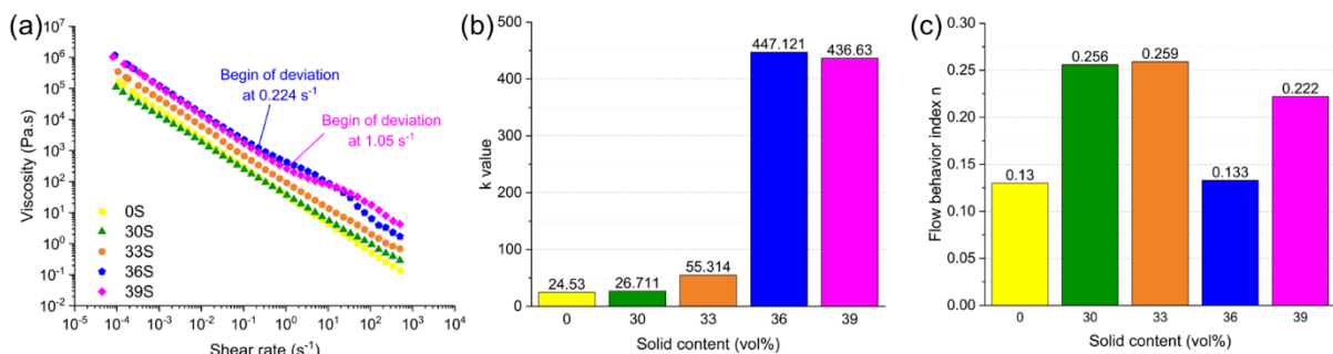
Fig. 31. (a) Viscosity \nu s. shear rate for varying solid contents. It is possible to observe the decrease of the viscosity as the shear rate increases, characteristic of pastes with shear-thinning behavior. The value of shear rate at which the viscosity values deviate from a linear decrease (acknowledging the logarithmic scale) are displayed for the two pastes that present this deviation. Values of (b) k and (c) n of the Ostwald-de Waele power law for the different solid contents evaluated.
